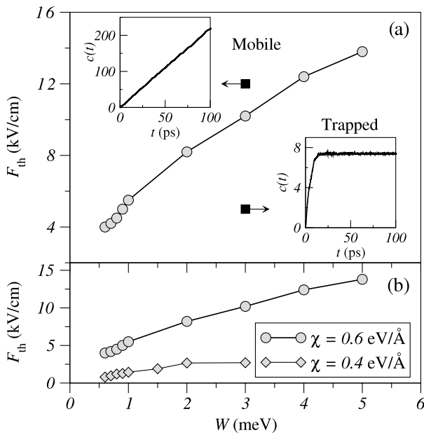
Figure 3. (a) Threshold electric field, F_{th} , above which the polaron becomes mobile, as a function of the magnitude of disorder for \chi = 0.6 \text{ eV \AA}^{-1} . The insets show the centroid as a function of time for the values of electric field and magnitude of disorder marked by solid squares. (b) Comparison of the threshold electric field, F_{th} , for \chi = 0.4 and 0.6 \text{ eV \AA}^{-1} .
